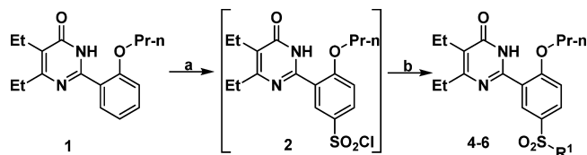
Scheme 1. Synthesis of Compounds 4–6 a
